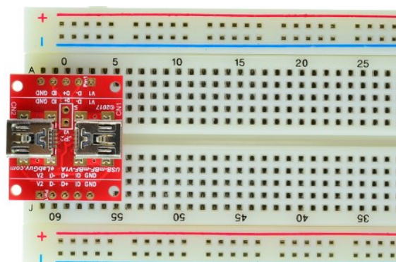
Figure 2: Example of connecting the USB-mBF-mBF-V1A on a breadboard (Note: This picture only shows the pins spacing, actual use may not be used on a breadboard)
